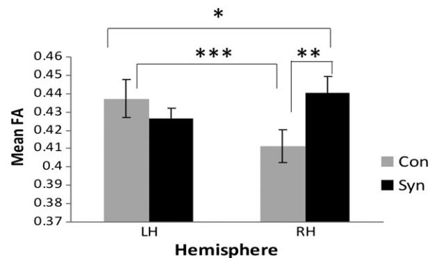
Fig. 3. Main comparisons in mean FA of the IFOF. Bars represent means. Error bars represent standard error. *Group \times hemisphere interaction: p < 0.05 ; **between-group difference: p < 0.05 ; ***inter-hemispheric difference: p < 0.01 (post-hoc Tukey's HSD).
